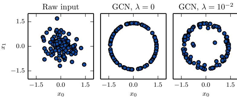
Figure 12.1: GCN maps examples onto a sphere. ( Left ) Raw input data may have any norm. ( Center ) GCN with \lambda = 0 maps all nonzero examples perfectly onto a sphere. Here we use s = 1 and \epsilon = 10^{-8} . Because we use GCN based on normalizing the standard deviation rather than the L^2 norm, the resulting sphere is not the unit sphere. ( Right ) Regularized GCN, with \lambda > 0 , draws examples toward the sphere but does not completely discard the variation in their norm. We leave s and \epsilon the same as before.
